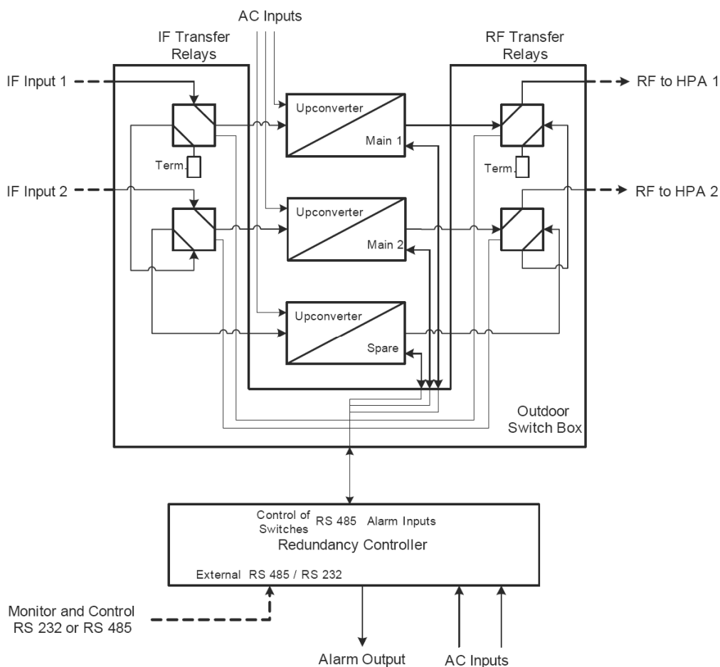
2:1 Redundancy Switch System with Outdoor Switch Unit
