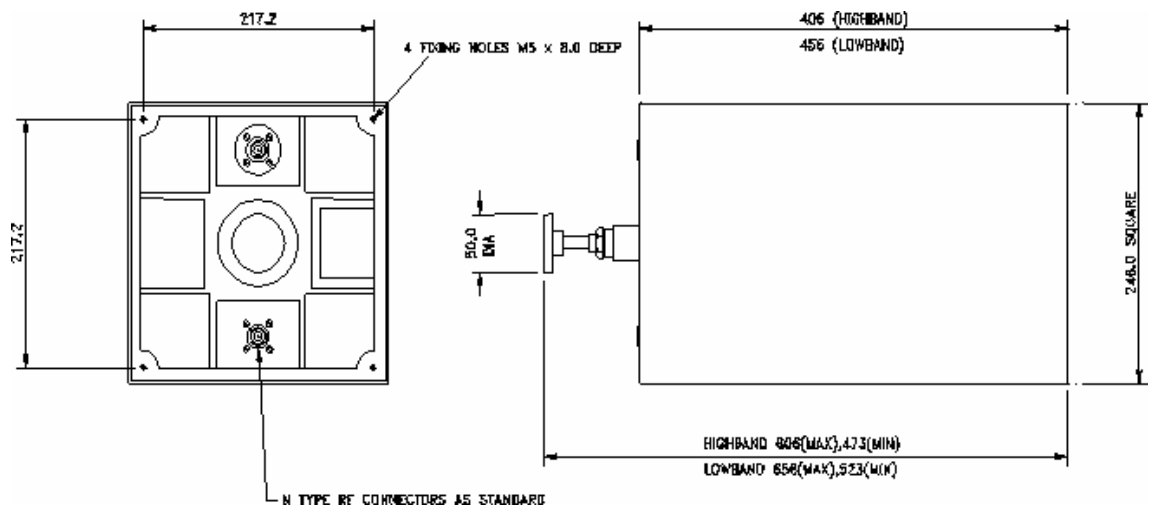
VHF Cavity general arrangement
